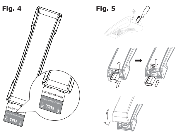
Fig. 4: Removing the battery cover and inserting the battery pack.
